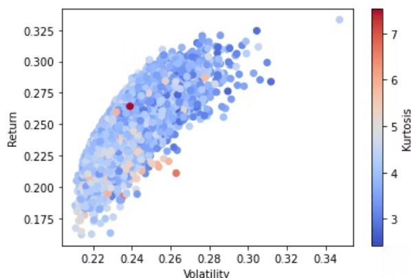
Figure 5: 10,000 Simulated Portfolios and Their Kurtosis
