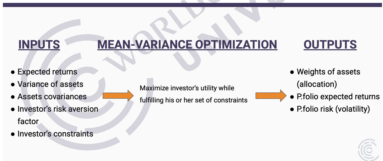
Figure 1. Mean-variance optimization and how it works.
